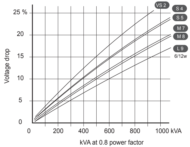
Load application (AREP or PMG excitation)
